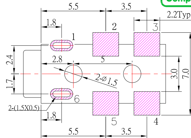
P.C.B LAYOUT MOUNTING PATTERN (TOP VIEW)
