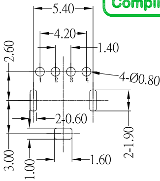
PCB LAYOUT
