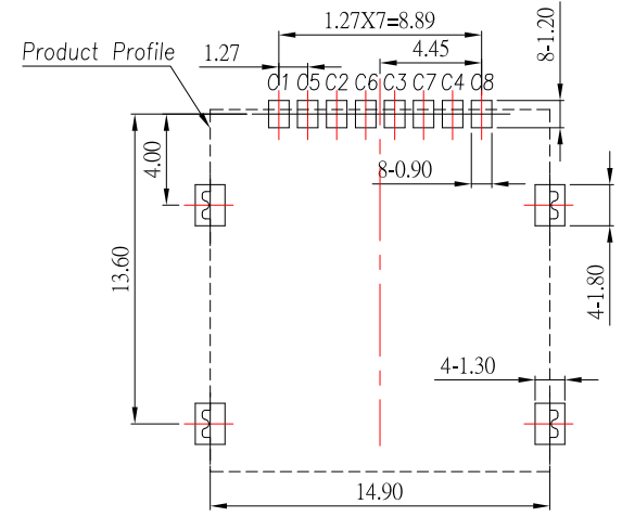
PCB LAYOYT
