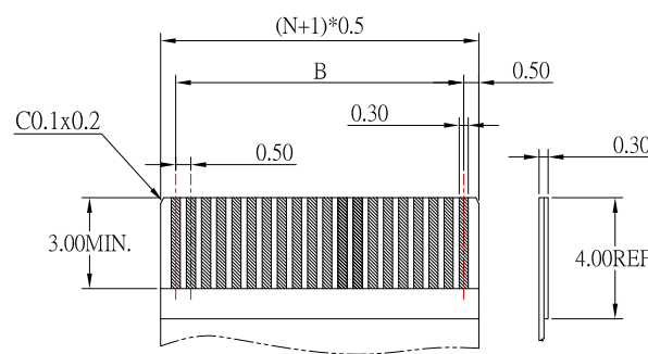
APPLICABLE FPC/FFC
