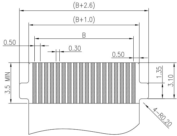
APPLICABLE FPC/FFC
