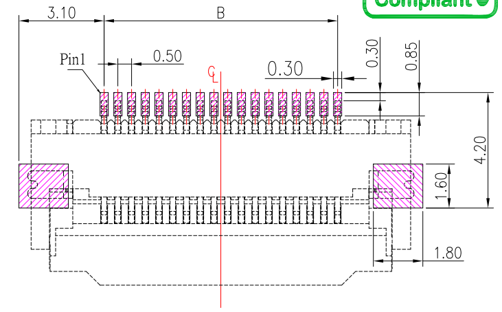
PCB LAYOUT
