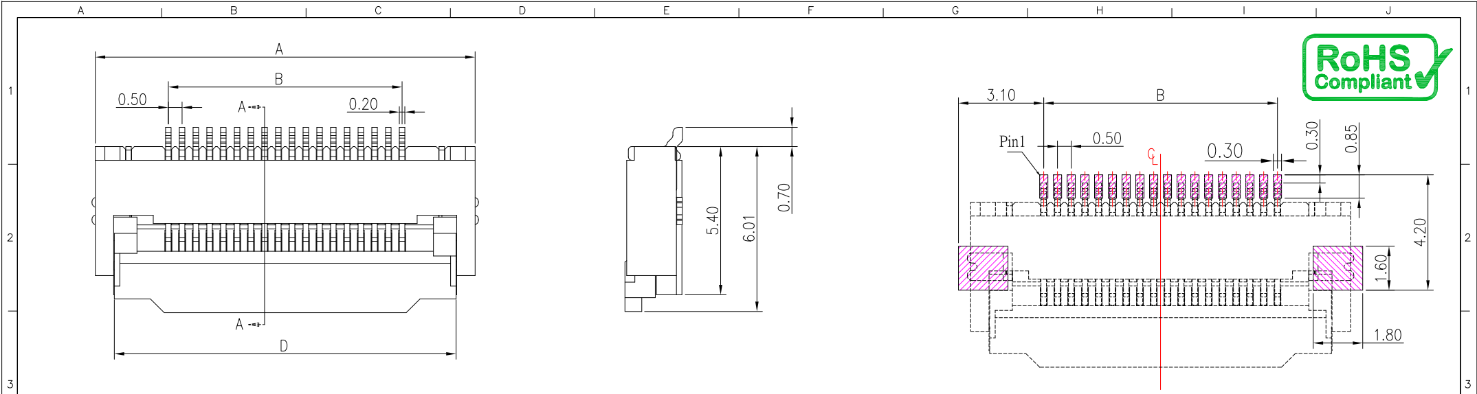
PCB LAYOUT
