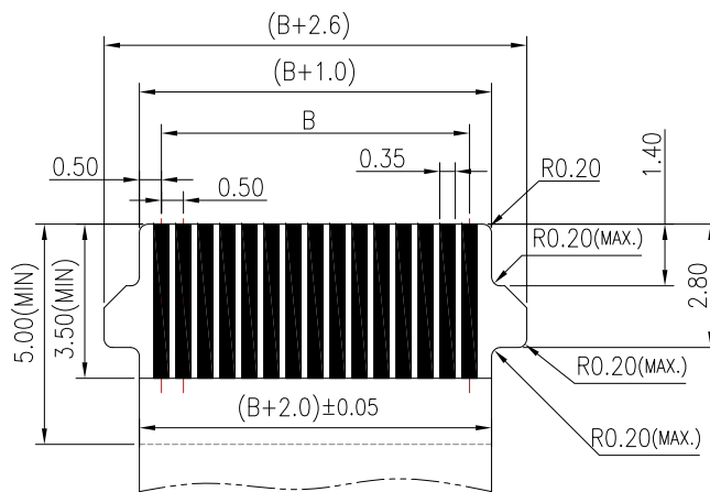
APPLICABLE FPC/FFC
