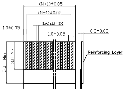
RECOMMENDED FFC/FPC DIM.
