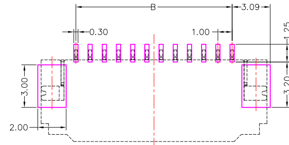
FPC/FFC Insert Direction
