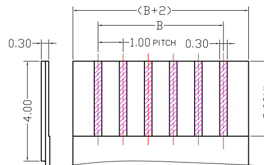
Applicable FPC
