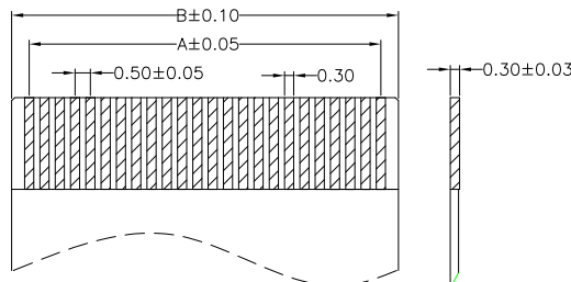
RECOMMENDED FPC DIMENSION
