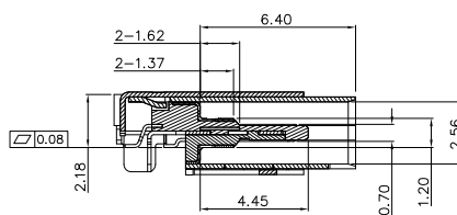
SECTION B-B SCALE 1:1
