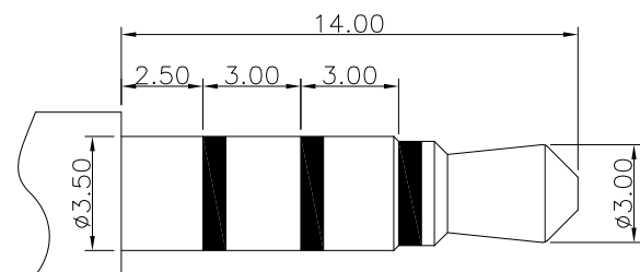
φ3.50mm 4 POLE PLUG
