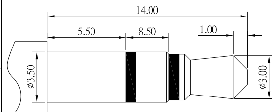
3.5mm 3 POLE PLUG
