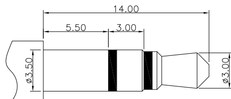
3.50mm 3 POLE PLUG
