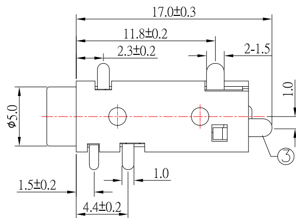
SCHEMATIC
