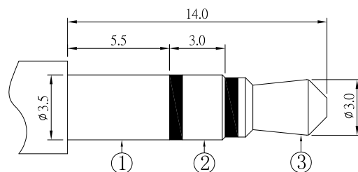
ø3.50mm 3 POLE PLUG
