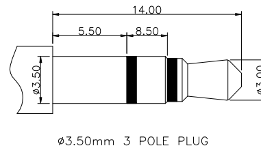
Ø3.50mm 3 POLE PLUG
