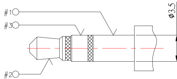
3.5 MATE PLUG
