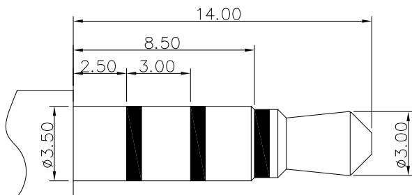
Ø3.50mm 4 POLE PLUG
