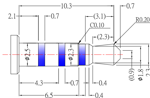
φ2.50mm 4 POLE PLUG DETAIL DRAWING
