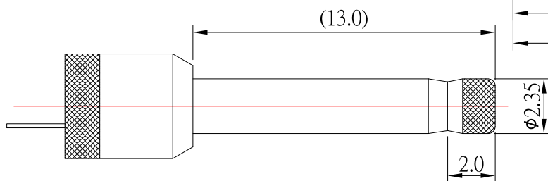
RECOMMENDED PLUG
