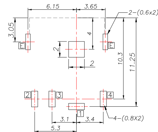
PCB LAYOUT MOUNTING PATTENR (BOTTOM VIEW)
