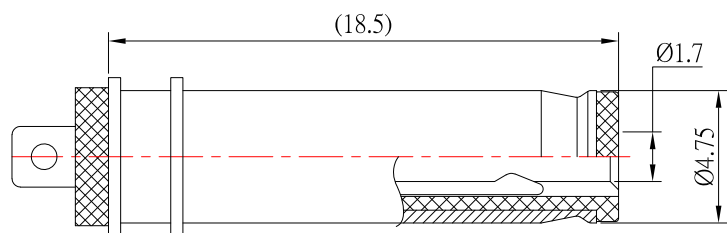
RECOMMENDED PLUG
