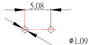
P.C.MOUNTING
