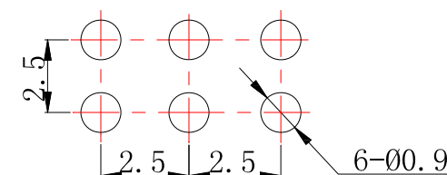
P.C.B LAYOUT MOUNTING PATTERN
