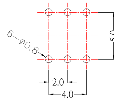
P.C.B MOUNTING PATTERN
