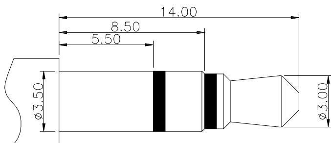
ø3.50mm 3 POLE PLUG
