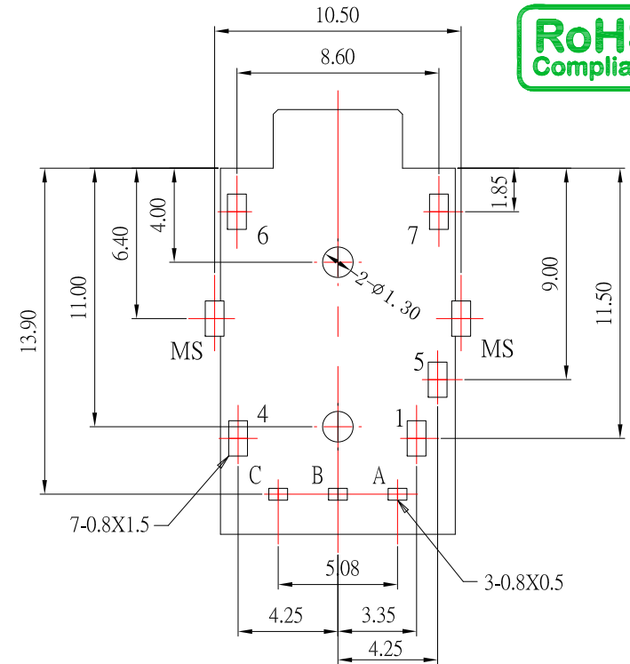
Recommended PCB Layout <BOTTOM VIEW>
