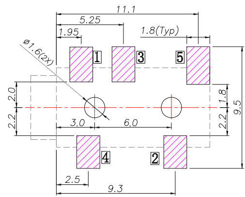
RECOMMENDED P. C. B. LAYOUT (COPPER-SIDED VIEW)
