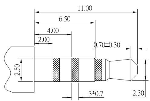
Ø2.50mm 4 POLE PLUG
